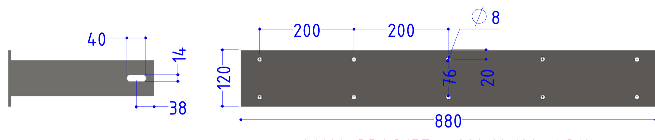
WALL BRACKET - 880 X 120 X 310
