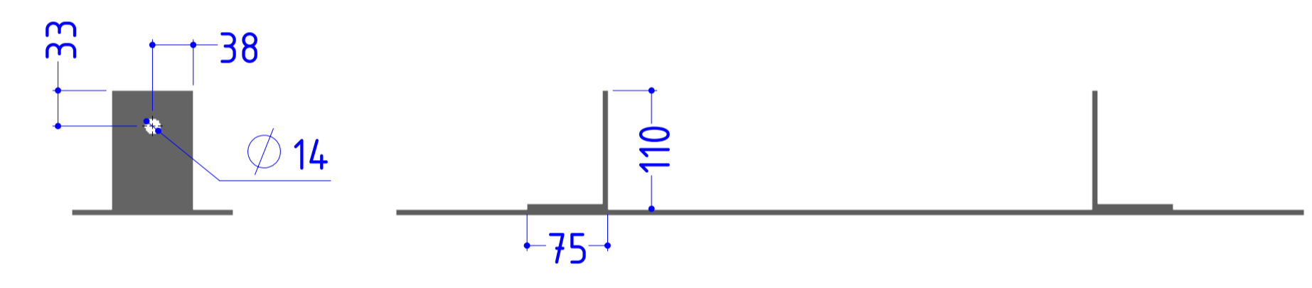
SPREADER PLATE-L BRACKET
